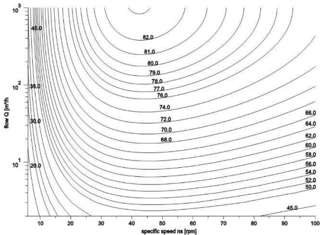
MEI = 0.4 for ESOB 2900 rpm
